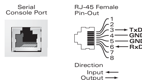
Figure 5 Serial Port Pin-Out
