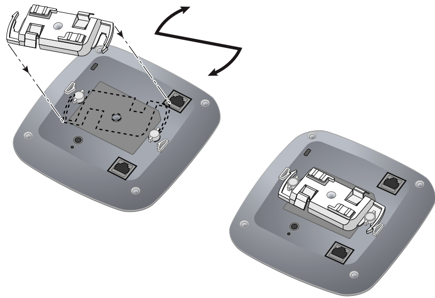
Figure 7 Attaching the Ceiling Rail Adapter
